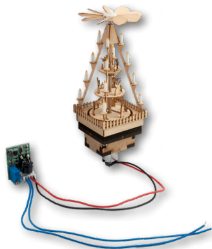
H0 66413 micro-motion Christmas Market Pyramid 4.5 x 4.5 cm, 9 cm high, installation depth 4 cm
