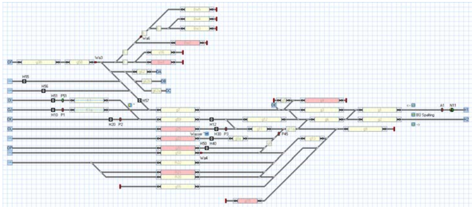
Diagram 53: Switchboard Example
