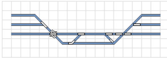
Diagram 66: Normal and Space saving Turnouts
