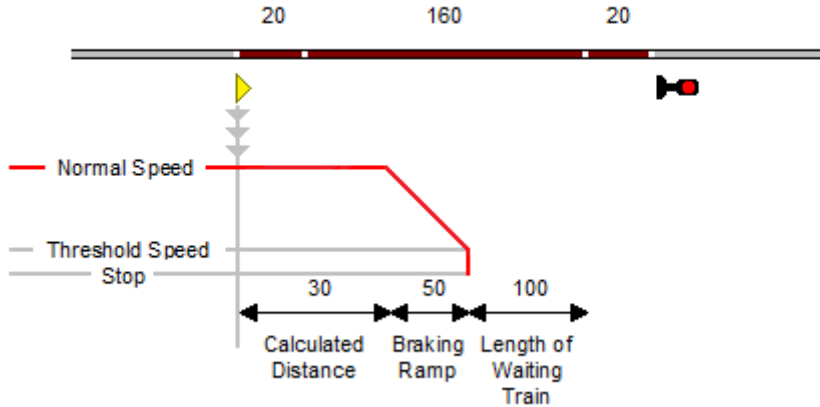
Diagram 151: Stopping for Coupling
