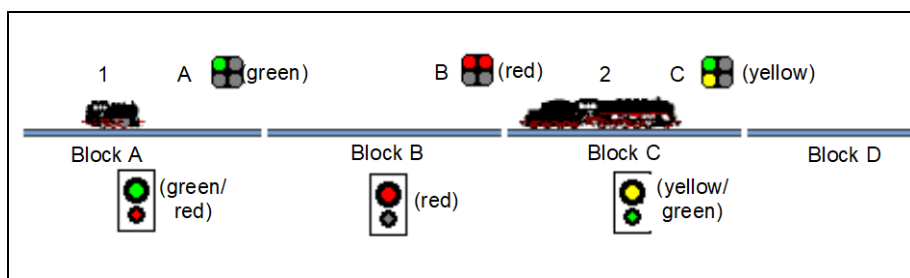
Diagram 121: Block Signals
