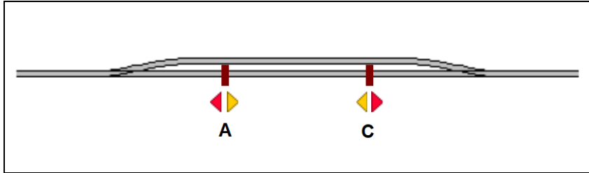
Diagram 112: Simple Block with two momentary sensors
